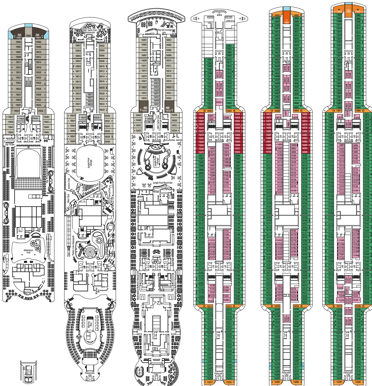
DEK 19 SIR BANI YAS
